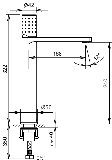
C36116 Single Lever Extended Height Basin Mixer without Pop-up Waste Set, Swivel Aerator
