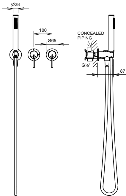
C36927 Single Lever Concealed Shower Mixer with 2-way manual diverter (handshower and headshower mode), complete with shower hose (1500mm), handshower and headshower
