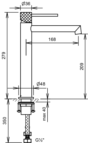
C36126 Single Lever Extended Height Basin Mixer without Pop-up Waste Set
