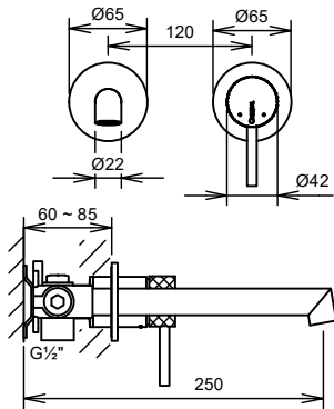
C36920 Single Lever Wall Mounted Basin Mixer
