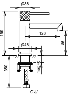
C36122 Single Lever Basin Mixer without Pop-up Waste Set
