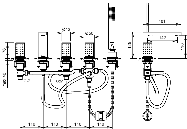
C20550 5-Hole Bath Shower Mixer with manual diverter, swivel aerator, complete with handshower and shower hose
