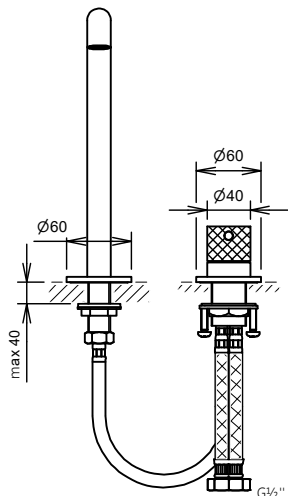
C36129 2-Hole Basin Mixer without Pop-up Waste Set
