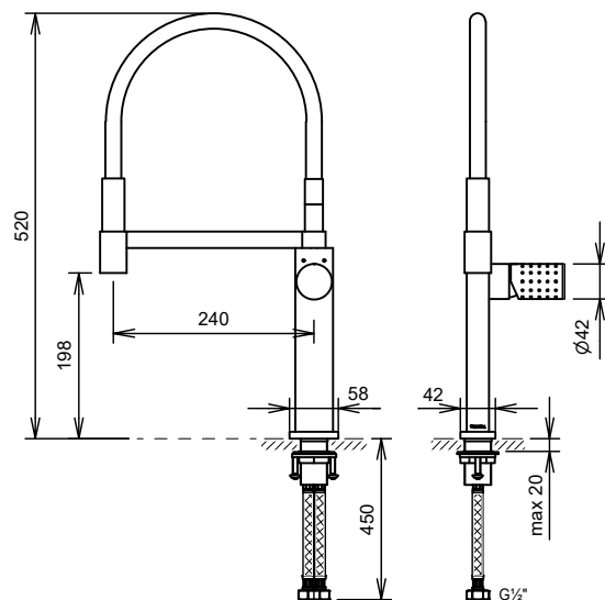
C36786 Single Lever Sink Mixer with swivel spout and pull-out handspray
