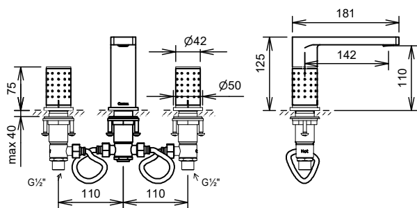
C20351 3-Hole Basin Mixer without Pop-up Waste Set, Swivel Aerator
