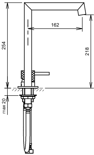
C36129 2-Hole Basin Mixer without Pop-up Waste Set
