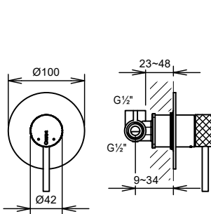
C36921 Single Lever Concealed Shower Mixer
