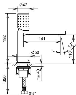
C36112 Single Lever Basin Mixer without Pop-up Waste Set, Swivel Aerator
