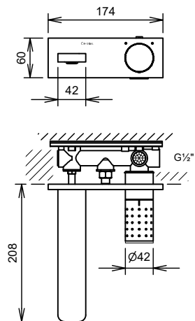
C36910 Single Lever Wall Mounted Basin Mixer, Swivel Aerator
