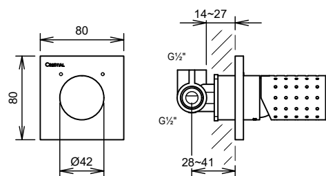
C36911 Single Lever Concealed Shower Mixer
