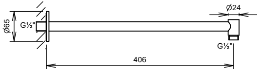
C28635 Shower arm
